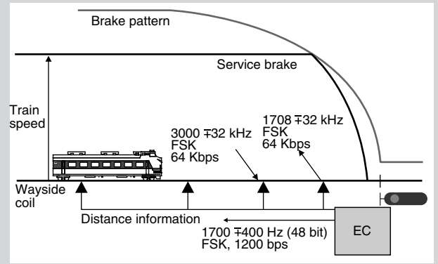
Figure 4 ATS-P Operating Principle
