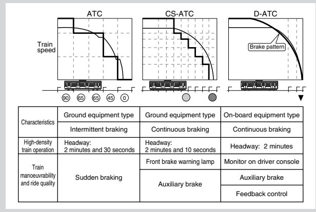
Figure 8 Performances of Train Control Systems
