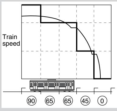
Figure 5 ATC Operating Principle
