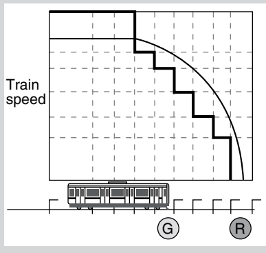
Figure 6 ATC with Continuous Braking Control Operating Principle
