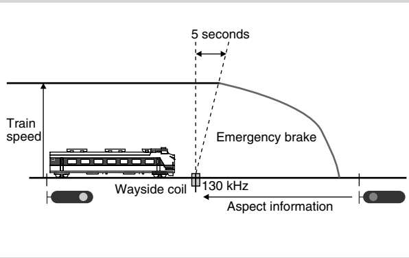
Figure 3 ATS-S Operating Principle
