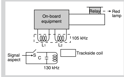
Figure 2 Operating Principle of Cab Warning System
